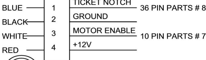
Ticket Dispenser Connection Diagram
